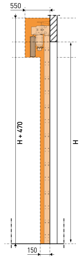
[ Cross section ]
