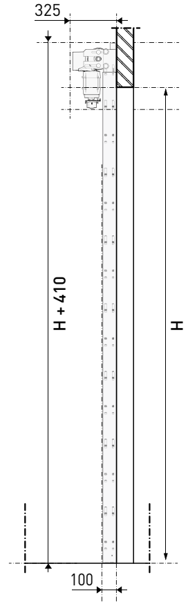
[ Cross section ]
