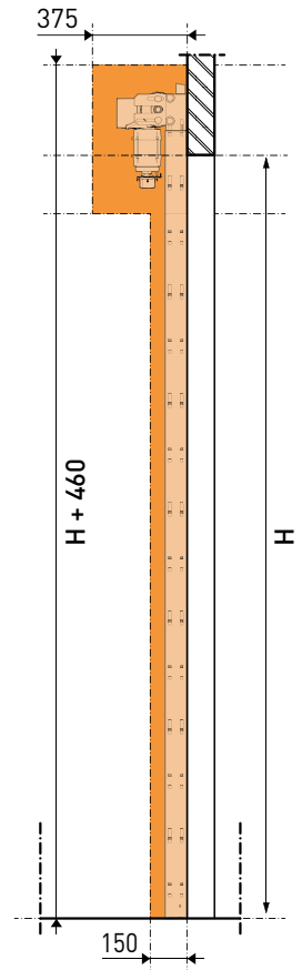
[ Cross section ]
