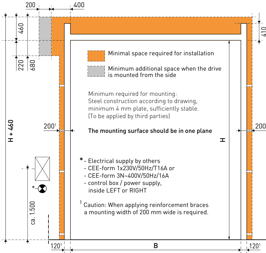
[ Drive side ]
