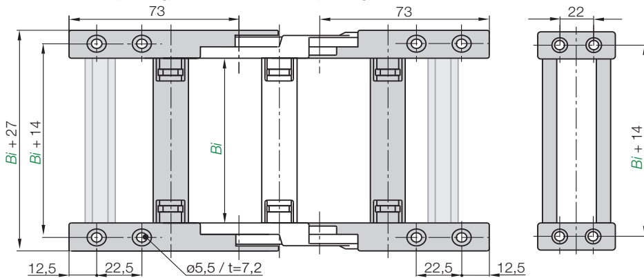
28280/77280...2 (pivoting) 29280/78280...2 (locking)
