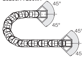
Fixed end 28280/77280...2
